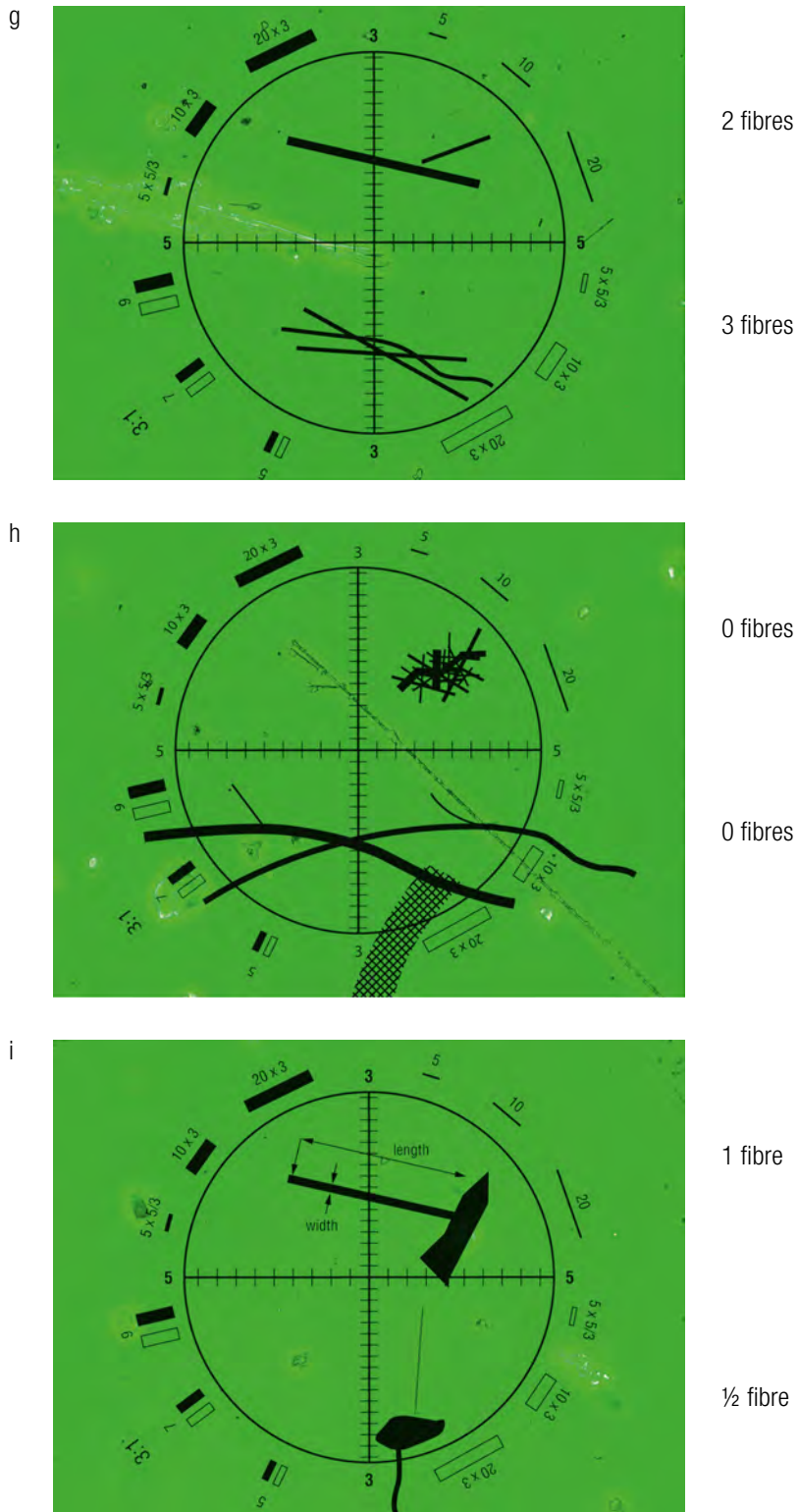
Figure A1.10 g-i Examples of fibre-counting rules for grouped fibres
